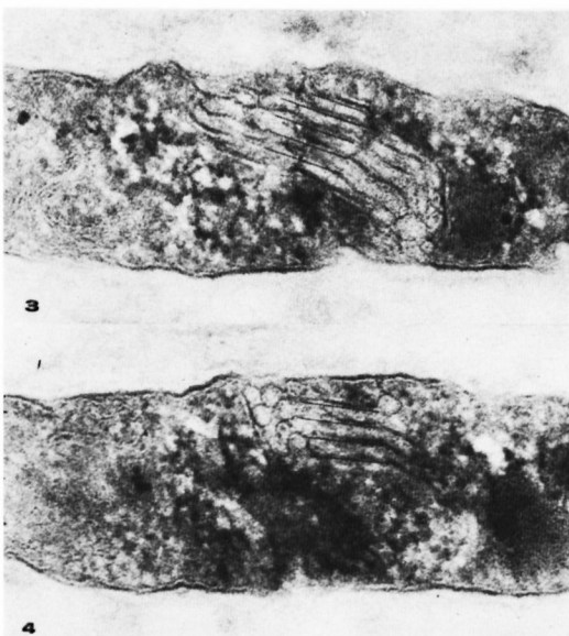
FIG. 5b. High magnification of Figure 5a. Photos 3-4. The black lines show the laminar membranous structures.
