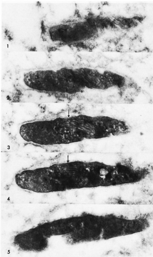
FIG. 5a. Longitudinal serial thin sections. The mesosome depicted in these serial sections shows bizarre structures.
