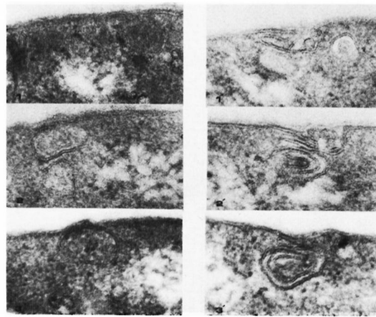
FIG. 6. A series of three sections demonstrating the expansion and distention of the mesosome.
