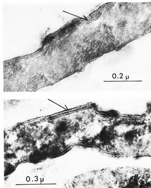
FIGS. 1a, 1b. Longitudinal thin sections. Arrows show the trilaminar membranous structures parallel to the bacillary cell envelope.
