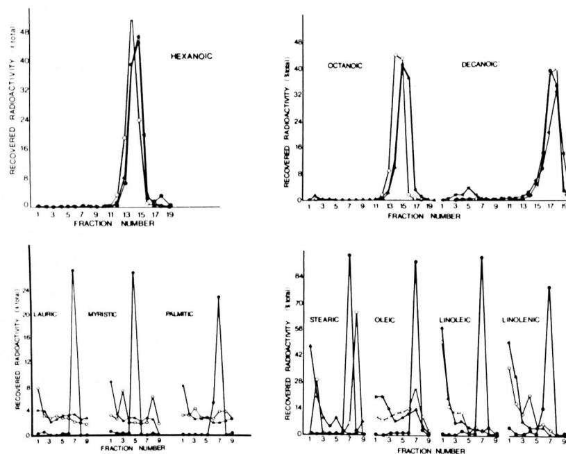
FIG. 3. Radiochromatogram of M. lepraemurium suspending buffer (K-36) containing [1- 14 C] hexanoic, or octanoic, or decanoic, or lauric, or myristic, or palmitic, or stearic, or oleic, or linoleic, or linolenic acid, after 5 days of incubation. ▲ Experimental vials. ● Standard substrate. ○ Control vials.
