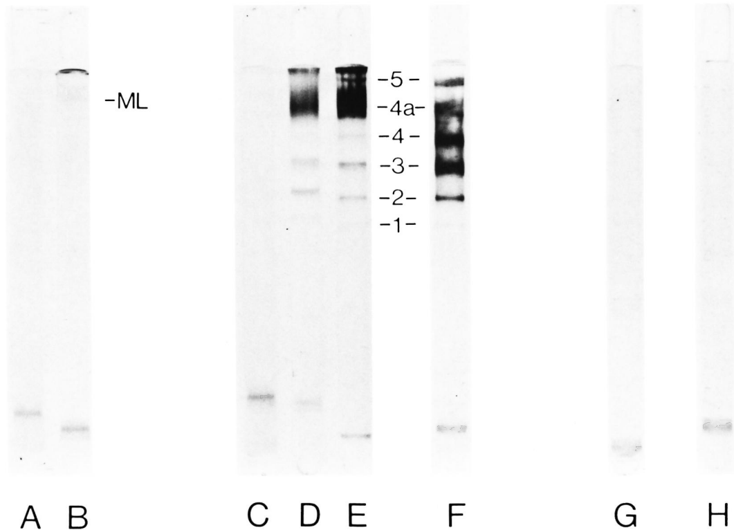
THE FIGURE. Polyacrylamide gel electrophoresis of lactate dehydrogenase in cell-free extracts. Tracks A, B, G & H = extracts from untreated M. leprae 3 (1.2 mg protein). Tracks C, D & E = extracts from uninfected armadillo liver (0.2 mg protein). Track F = extract from infected armadillo liver (0.6 mg protein).
