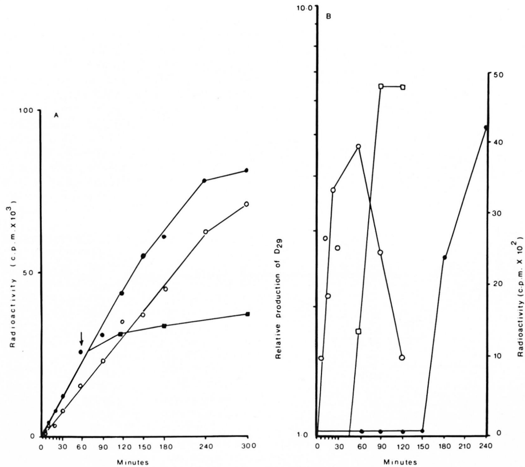
FIG. 3. Incorporation of leucine-U- 14 C in proteins in noninfected and D 29 -infected M. tuberculosis . A) Time course of incorporation in noninfected (●—●) and D 29 -infected (○—○) bacilli; (■—■) represents the inhibition of protein synthesis caused by the addition of 50 μg/ml of streptomycin (arrow) to noninfected bacilli (control to verify if incorporation was truly into proteins). B) Composite figure representing the one-step growth of D 29 in tubercle bacilli (●—●); premature lysis induced by streptomycin (□—□); and the incorporation of radiolabeled leucine in the proteins of D 29 -infected bacilli during a premature lysis experiment in the presence of streptomycin and D-cycloserine (○—○). D-cycloserine was added to potentiate phage-induced lysis.
