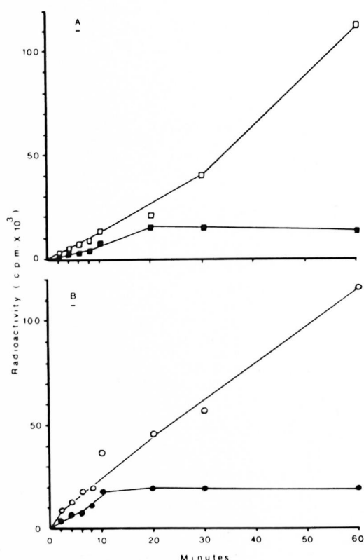
FIG. 4. Incorporation of acetate-2- 14 C into the lipids of noninfected and D 29 -infected bacteria. A) M. smegmatis . Noninfected (□—□), D 29 -infected (■—■). B) M. tuberculosis . Noninfected (○—○), D 29 -infected (●—●).
